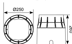
Installation Sleeve
