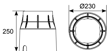
Installation Sleeve
