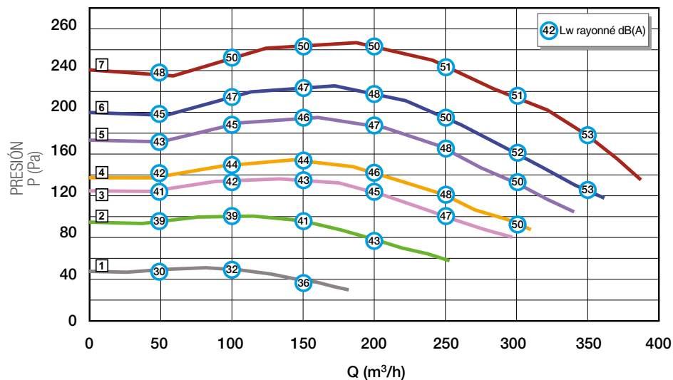
EasyHOME Hygro Compact Premium SP
