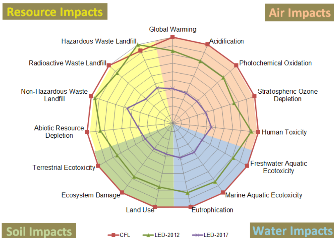
Figure 7-6. Life-Cycle Assessment Impacts of the Lamps Analyzed Relative to CFL
